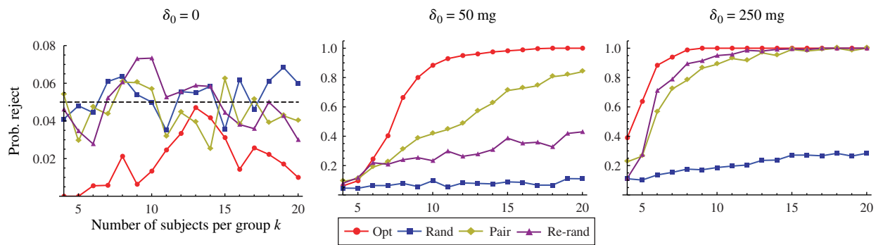
Figure 6. The probability of rejecting the null hypothesis of no effect for various effect sizes.
